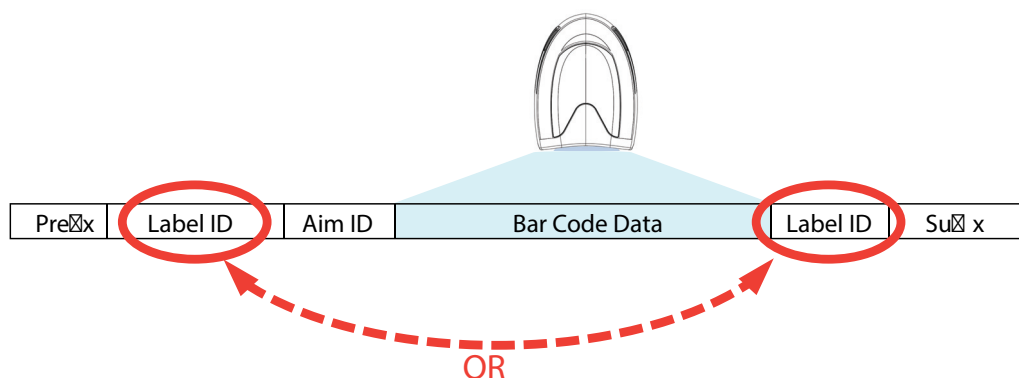
Figure 19 Label ID Position Options
